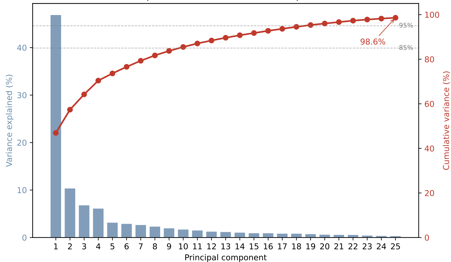
PCA Explained Variance (40 → 25 components)
